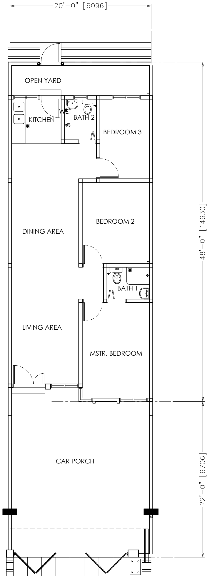
FLOOR PLAN
